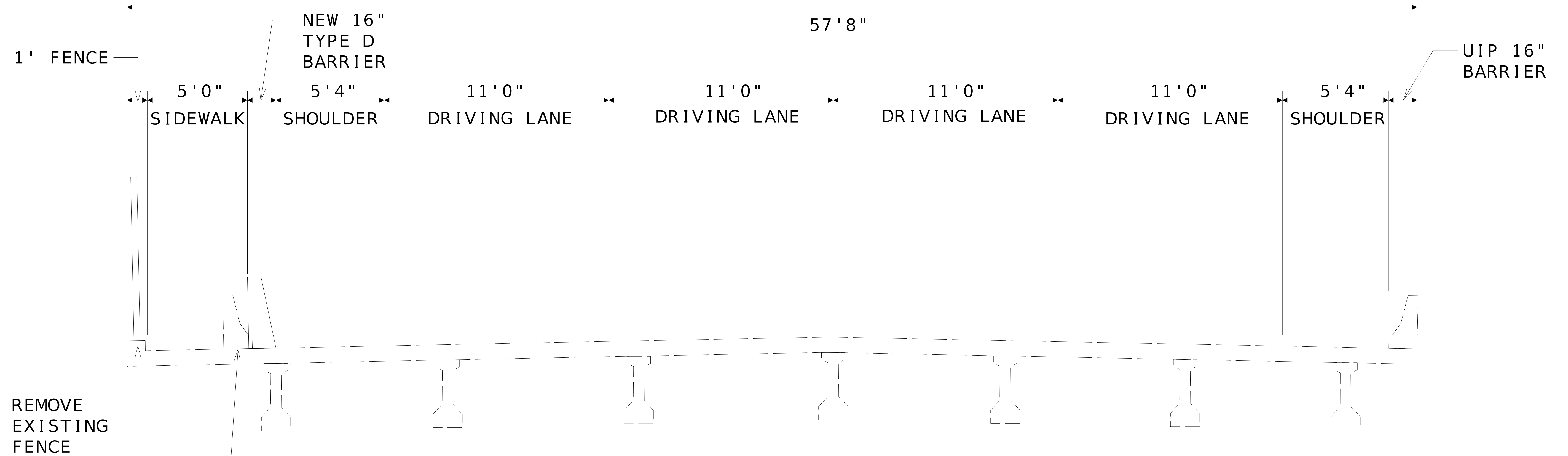
BRIDGE A5961 TYPICAL SECTION OVER CPKC RAILROAD, MNA RAILROAD, JOPLIN CREEK
