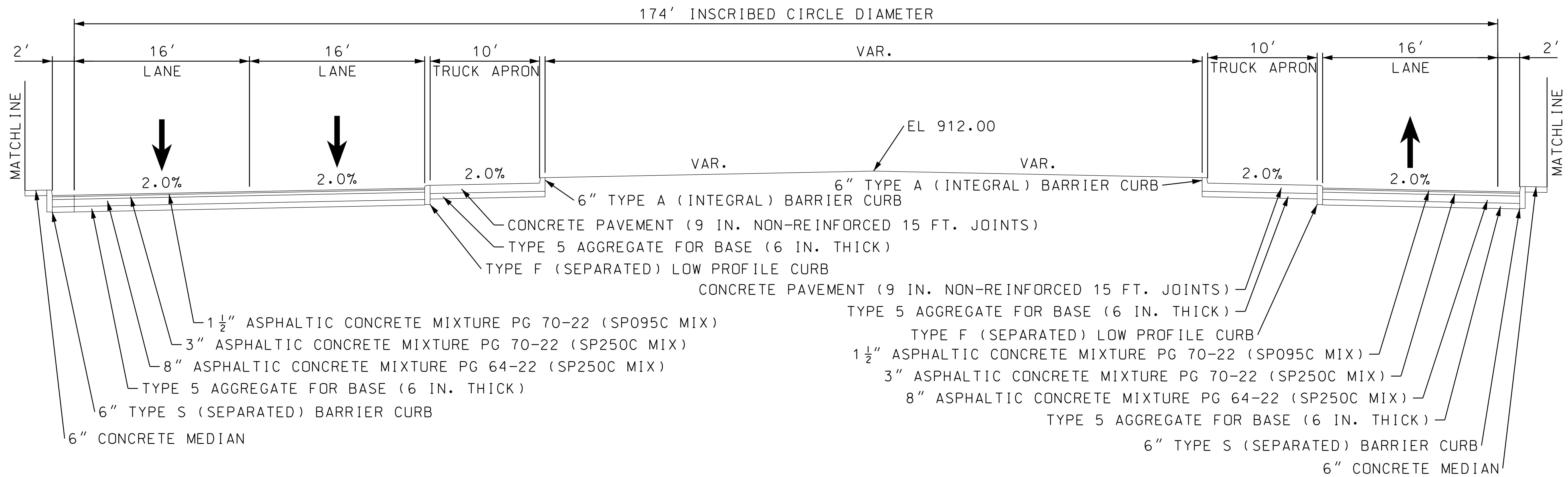
PROPOSED TYPICAL SECTION ROUNDBOUT
