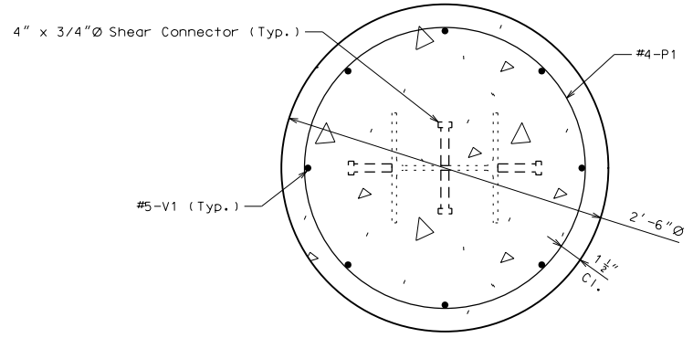
SECTION SHOWING PILE ENCASEMENT PILE ENCASEMENT
