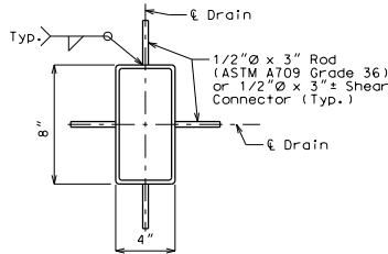
PLAN OF STEEL DRAIN OPTION
