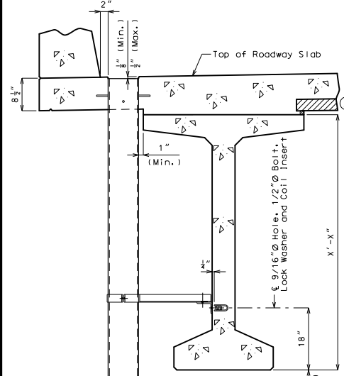
PART SECTION NEAR DRAIN
