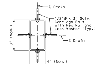
PLAN OF FRP DRAIN OPTION
