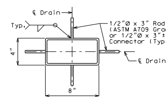
PLAN OF STEEL DRAIN OPTION
