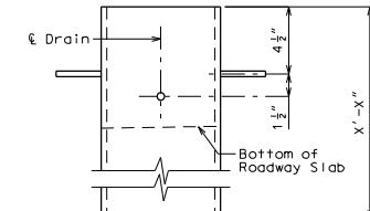
ELEVATION OF DRAIN
