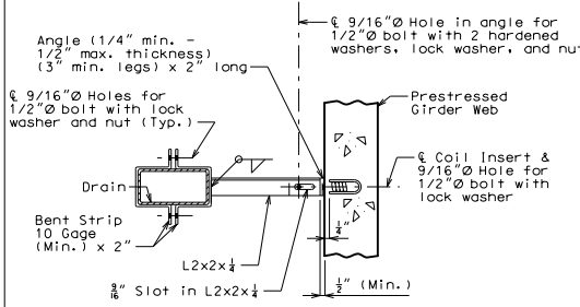
PART SECTION SHOWING BRACKET ASSEMBLY
