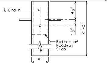
ELEVATION OF DRAIN
