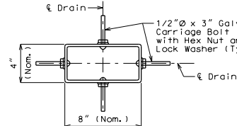
PLAN OF FRP DRAIN OPTION
