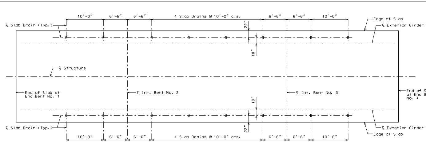
PLAN OF SLAB SHOWING SLAB DRAIN LOCATIONS
