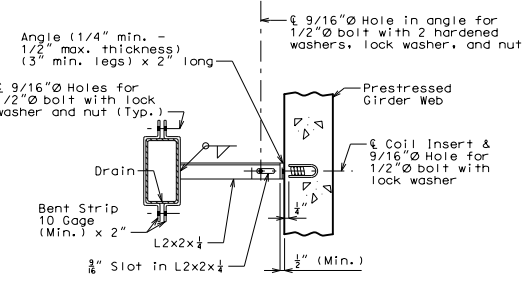
PART SECTION SHOWING BRACKET ASSEMBLY
