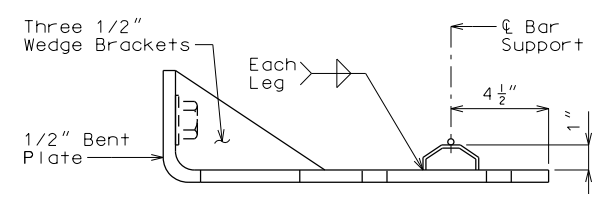
PART SECTION THRU PLATE
