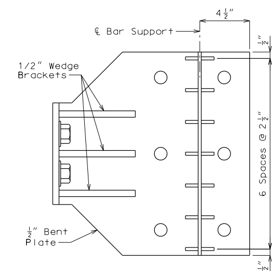
PLAN OF BENT PLATE
