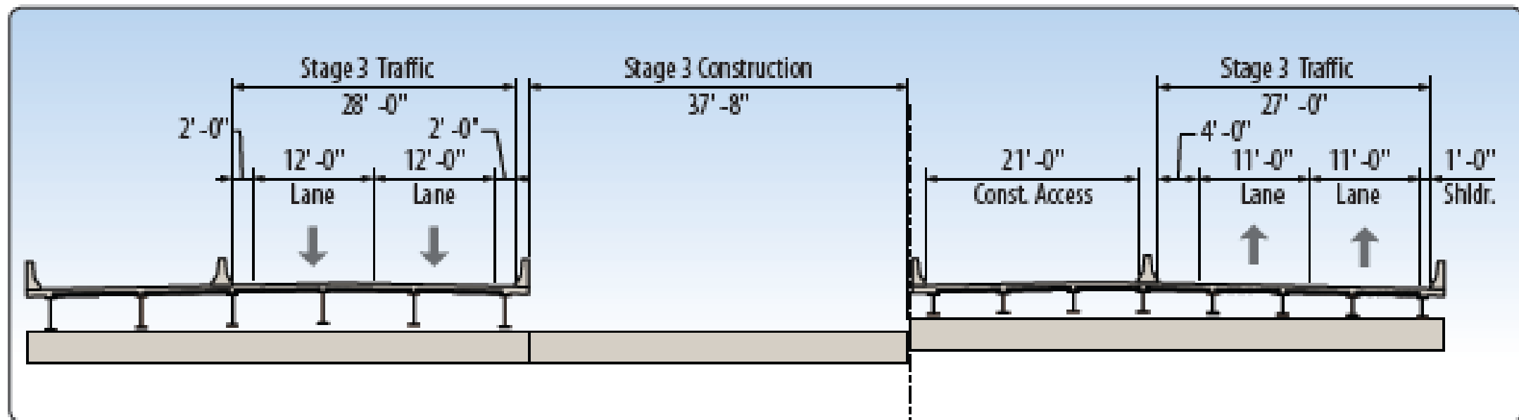
I-70 over Garth Avenue Phasing Typical Section
