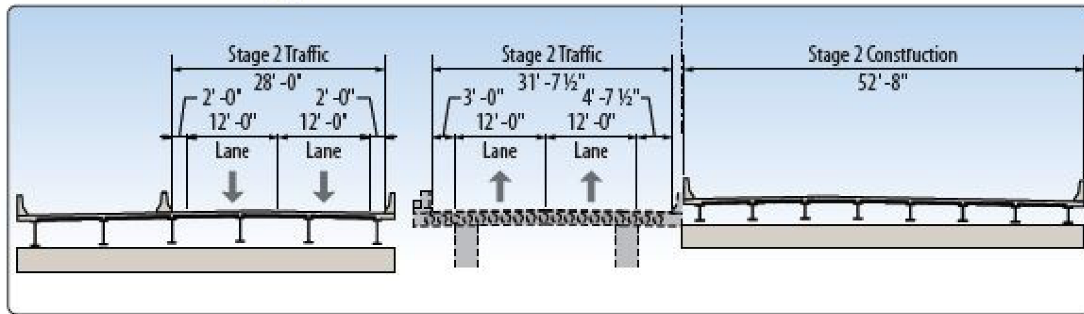
I-70 over Garth Avenue Phasing Typical Section
