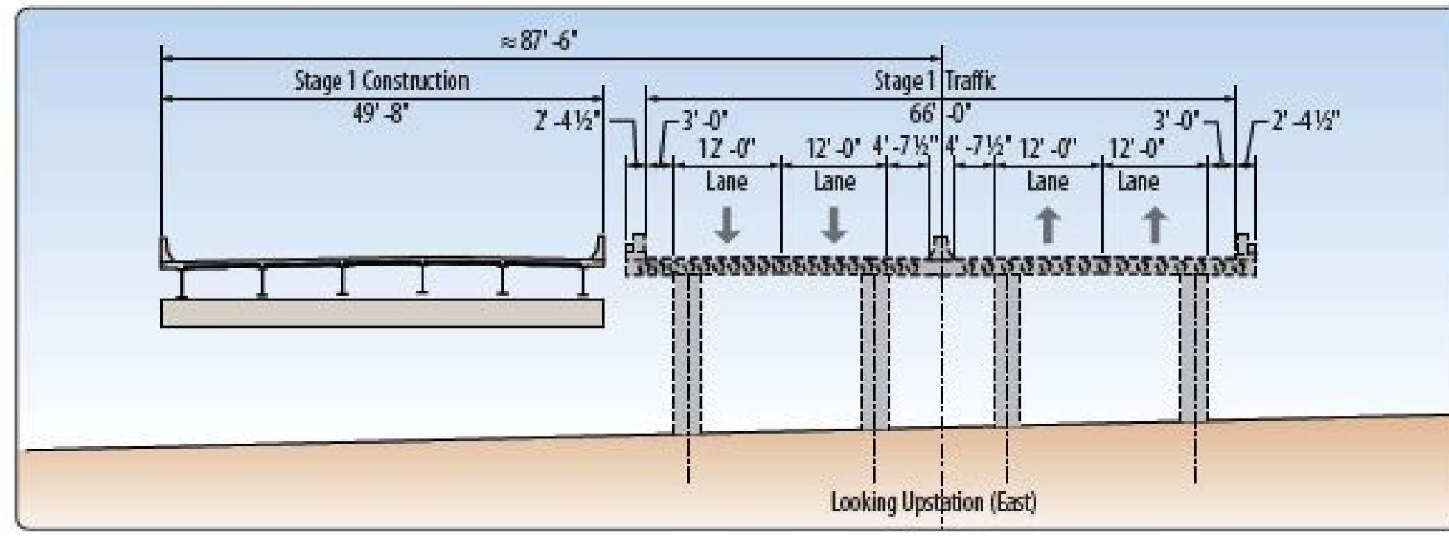
I-70 over Garth Avenue Phasing Typical Section
